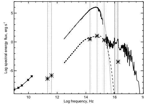
Fig. 2. The spectral energy distribution ( \nu f_\nu ) of the quiet Sun, with an optically thin warm chromospheric slab source superposed on the photosphere and shown as a dashed line. The parameters for this spectrum are 1.4 \times 10^4 \text{ K} , 10^{14} \text{ cm}^{-3} , emission measure 3 \times 10^{54} \text{ cm}^{-3} , and line-of-sight thickness 10^7 \text{ cm} . The visible/IR quiet-Sun data come from Wehrli (1985), the UV beyond 1200 \text{ \AA} from Warren (2005), and the microwave points from the Nobeyama fixed-frequency data for December 2008. The dotted line shows a blackbody at 5778 K. The flare points (asterisks) show data from Kaufmann et al. (2004), Xu et al. (2004), and our analysis of TRACE observations at 1600 \text{ \AA} and 171 \text{ \AA} , with all points scaled by the GOES magnitude of the event to a common X10 level.
